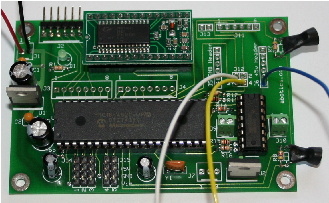
Figure 7. OPEN-ROBOT's PIC18F4520 Based Controller Board.
